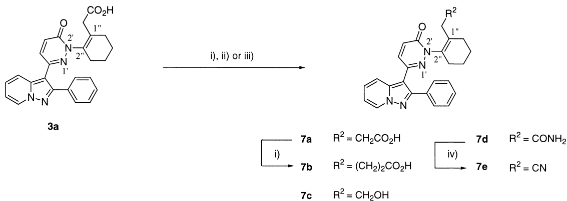
Scheme 2. Synthesis of N 2'-cyclohexenyl analogues. Reagents and conditions: (i) 1. SOCl 2 /CH 2 Cl 2 ; 2. trimethylsilyldiazomethane/THF–CH 3 CN; 3. 2,4,6-trimethylpyridine, PhCH 2 OH; 4. 1 N NaOH aq, THF–H 2 O ( 7a , 7b ). (ii) BH 3 ·THF, THF ( 7c ). (iii) 1-Ethyl-3-(3-dimethylaminopropyl)carbodiimide (EDC), HOBT, NH 4 Cl/THF–CH 2 Cl 2 ( 7d ). (iv) TFAA, pyridine, CH 2 Cl 2 ( 7e ).
