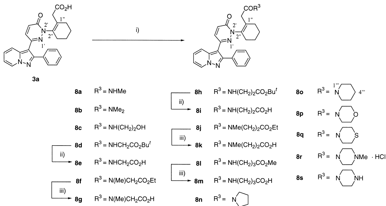
Scheme 3. Synthesis of amide derivatives of FR166124 ( 3a ). Reagents and conditions: (i) R^3\text{H}\cdot\text{HCl} , EDC, HOBT/THF- \text{CH}_2\text{Cl}_2 ( 8a , b , f , j , l ); R^3\text{H} , EDC \cdot\text{HCl} , HOBT/THF- \text{CH}_2\text{Cl}_2 ( 8c , p , q ) or DMF ( 8n , o ); (\text{COCl})_2/\text{DMF}-\text{CH}_2\text{Cl}_2 , then R^3\text{H}\cdot\text{HCl} , \text{Et}_3\text{N}/\text{CH}_2\text{Cl}_2 ( 8d , h ); R^3\text{H} , EDC \cdot\text{HCl} , HOBT, \text{Et}_3\text{N}/\text{DMF} , then 4 N HCl/EtOAc ( 8r ); 1-triphenylmethylpiperazine, EDC \cdot\text{HCl} , HOBT/THF- \text{CH}_2\text{Cl}_2 , then \text{HCO}_2\text{H} , c-HCl ( 8s ) (ii) TFA/ \text{CH}_2\text{Cl}_2 ( 8e , i ), (iii) 1 N NaOH/1,4-dioxane- \text{H}_2\text{O} ( 8g , k , m ).
